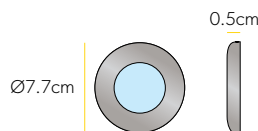
Cool White LED Showerlight Art No.: 5750
