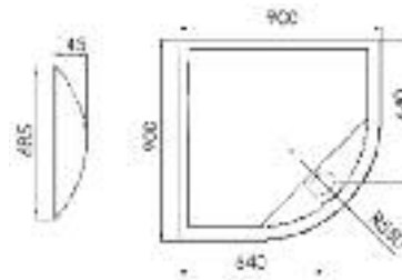
900 x 900mm Quadrant
