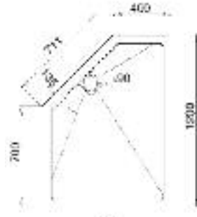
DNT129 Left Hand
