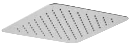
Square 300mm ceiling mounted stainless steel shower head 300(w) x 300mm(d) Minimum pressure 1.0bar
