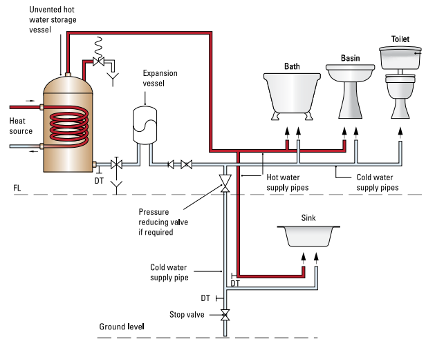
Figure 4 Pump Assisted
