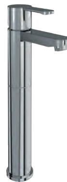
Tall basin mixer without pop-up waste 13.7cm x 5.2cm x 32.4cm CTA3 £249
