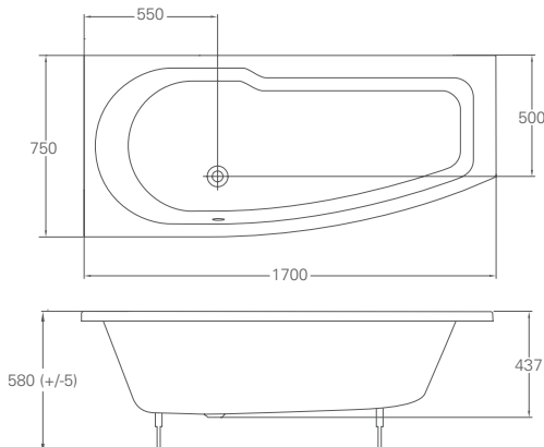
EcoCurve showering bath, page 130
