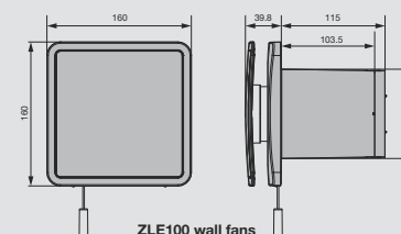
ZLE100 wall fans
