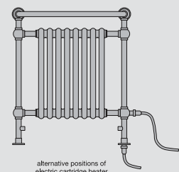
alternative positions of electric cartridge heater when specified
